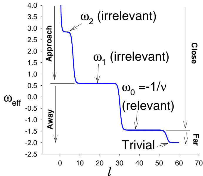
Figure 3. This figure is a continuation of figure 2. It shows the various plateaux that \omega_{\text{eff}}(l) undergoes along a RG trajectory first adjusted to approach f^* along the second irrelevant direction (plateau at \omega_2 = 2.84 ). Because it is not possible to exactly determine the initial conditions, the trajectory always ends up going away from the fixed point towards the trivial high temperature fixed point characterized by the classical value \frac{1}{2} (for minus the inverse of \omega_{\text{eff}}(l) , thus the final plateau at -2 ). In-between, the RG flow has been influenced by the close vicinity of the least irrelevant eigenvector (plateau at \omega_1 ) and that of the relevant eigenvector (plateau at \omega_0 = -\frac{1}{\nu} ). The various regimes of the RG flows are indicated by the vertical arrows on the left (direction of the flow with respect to the fixed point) and on the right of the figure (distance to the fixed point).
