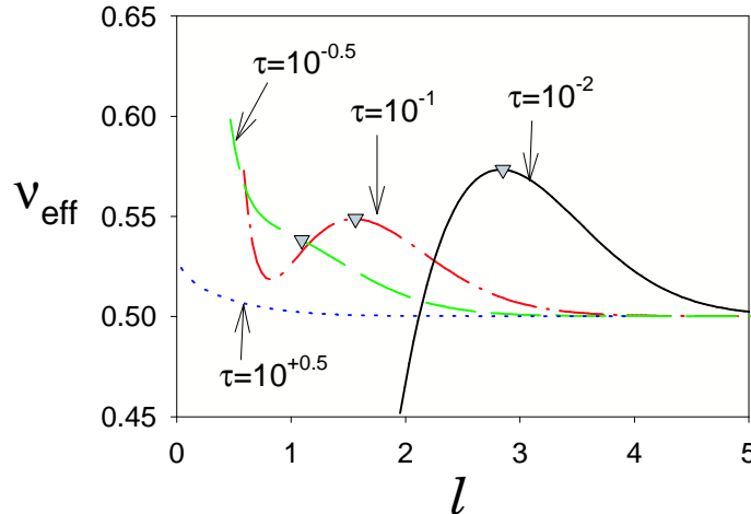
Figure 6. Illustration of the evolution of the extrema \nu_{\text{eff}}(l) [minus the inverse of equation (2.2)] for various values of \tau = (u_2(0) - u_2^c)/u_2^c and for the family of RG flows initialized at u_4(0) = 3 . The extremum (grey triangle) disappears at some not very large value of \tau (about 10^{-0.5} ) and does not reach the classical value \frac{1}{2} . This induces the partial Ising-to-classical crossover drawn in figure 5 (squares).
