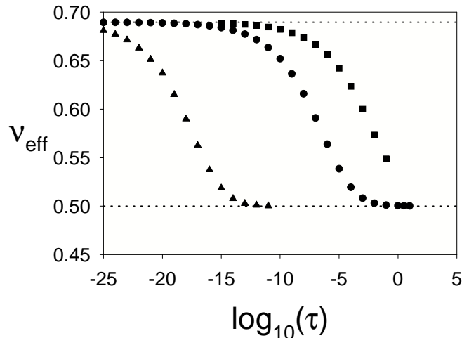
Figure 5. Evolutions of an effective exponent \nu_{\text{eff}}(\tau) [with \tau \propto (T - T_c)/T_c ] along three different families of RG trajectories (see text for additional details). The full squares indicate the evolution of \nu_{\text{eff}}(\tau) for a family of trajectories initialized in the sector u_4 > 0 with u_4(0) = 3 and for various values of u_2(0) (the same system at criticality corresponds to the white circle “Simple fluid” of figure 4). When u_2(0) \rightarrow u_2^c the effective exponent approaches the critical exponent value \nu \cong 0.69 compatible with the present study. One observes that the crossover towards the classical value \frac{1}{2} is not complete because \nu_{\text{eff}}(\tau) ceases to make sense before \tau becomes large. This is not the case of the evolution represented by the full circles which correspond to trajectories initialized close to the Gaussian fixed point. In this case the complete crossover reproduces the interpolation between the Gaussian and the Wilson-Fisher fixed points and typically corresponds to the usual answer given by field theory [28]. The third evolution (full triangles) corresponds to a family of Hamiltonian initialized close to the tricritical surface but still attracted to the Wilson-Fisher fixed point. One sees that the classical-to-Ising crossover is complete but highly retarded compared to the two other cases. This is because at criticality, the RG flow is first attracted to the Gaussian fixed point (showing then an apparent classical value of \nu ) before interpolating between the Gaussian and the Wilson-Fisher fixed point.
