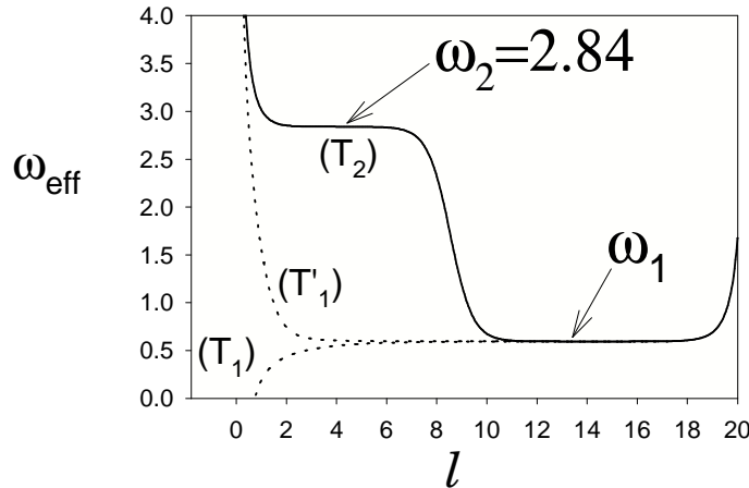
Figure 2. When a second condition is imposed on the initial Hamiltonian parameters, the approach to f^* may be adjusted such as to asymptotically take the second least irrelevant eigendirection. Here \omega_{\text{eff}}(l) is given by equation (2.2) for n = 2 it clearly undergoes (full line) a flat inflection point at the value \omega_2 = 2.84 corresponding to an approach to f^* along T_2 , the greater the critical parameter u_4^c is accurately determined the longer is the flat extremum. Because u_4^c is not completely determined [within the available accuracy in solving equation (2.1)] the trajectory leaves the direction of T_2 to take one of the two directions of approach associated to the least irrelevant inverse eigenvalue \omega_1 (corresponding to T_1 or T'_1 as indicated by dashed curves). Here, the trajectory corresponding to the full line goes along T'_1 . Again a flat extremum of \omega_{\text{eff}}(l) indicates the approach along an eigenvector of f^* and requires an accurate determination of the critical value u_2^c . Because this determination is not complete, the trajectory ends up going away from f^* as indicated by the sudden departure of \omega_{\text{eff}}(l) from \omega_1 for the large values of l .
