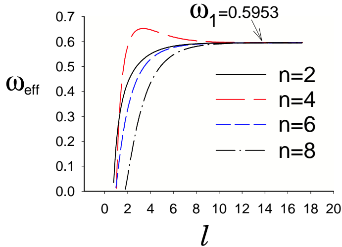
Figure 1. Evolutions for d = 3 of the first four Hamiltonian parameters u_2(l) , u_4(l) , u_6(l) , u_8(l) in a close approach to the Wilson-Fisher fixed point f^* along T_1 or T'_1 . The effective inverse eigenvalue \omega_{\text{eff}}(l) is given by equation (2.2) for n = 2, 4, 6, 8 . All these quantities reach the same universal value \omega_1 characteristic of the least irrelevant eigendirection of f^* . To get this close approach to f^* from equation (2.1), the initial critical value u_2^c corresponding to u_4(0) = 3 , has been determined with more than twenty digits.
