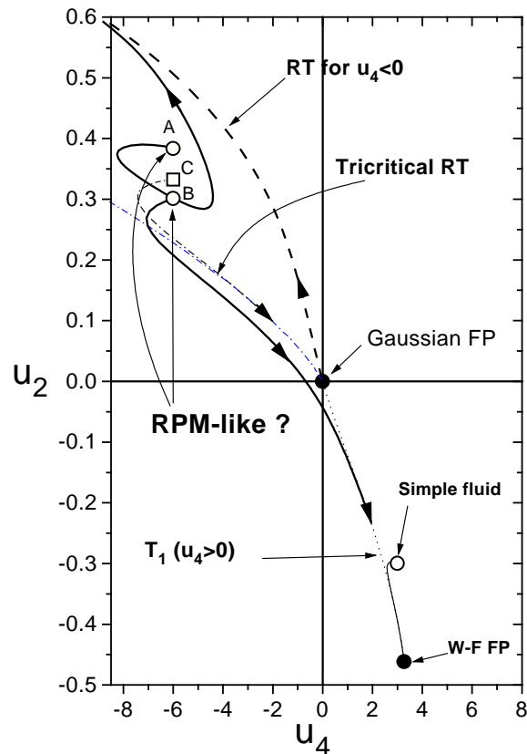
Figure 4. Domains of attraction and repulsion of the Gaussian fixed point. The figure represents projections onto the plane \{u_2, u_4\} of various RG trajectories running in the space S minus one dimension. The flows have been obtained by solving equation (2.1). Black circles represent the Gaussian and the Wilson-Fisher (W-F FP) fixed points. The arrows indicate the directions of the RG flows on the trajectories. The ideal trajectory (dot line) which interpolates between these two fixed points represents the usual renormalized trajectory T_1 corresponding to the so-called \varphi_3^4 renormalized field theory in three dimensions (usual RT for u_4 > 0 ). White circles represent the projections onto the plane of initial critical Hamiltonians. For u_4(0) > 0 , the effective Hamiltonians run toward the Ising fixed point asymptotically along T_1 (simple fluid). Instead, for u_4(0) < 0 and according to the values of Hamiltonian coefficients of higher order ( u_6, u_8 , etc.), the RG trajectories either (A) meet an endless RT emerging from the Gaussian FP (dashed curve) and lying entirely in the sector u_4 < 0 or (B) meet the usual RT T_1 to reach the Ising fixed point. The frontier which separates these two very different cases (A and B) corresponds to initial Hamiltonians lying on the tricritical subspace S_t (white square C). This is a source of RG trajectories flowing asymptotically toward the Gaussian FP along the tricritical RT. Notice that the coincidence of the initial point B with the RG trajectory starting at point A is not real (it is accidental, due to a projection onto a plane of trajectories lying in a space of infinite dimension). The points A or B could correspond to the restricted primitive model of ionic systems (see [8]).
