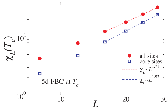
Figure 2. (Color online) FSS for the 5D Ising susceptibility at the critical point T_c from all sites (upper red data) and core sites (lower blue data). Neither Gaussian nor Q -FSS is supported (see also figure 5 (a) of reference [4]).
