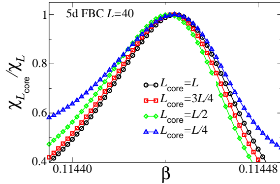
Figure 4. (Color online) The value of the pseudocritical temperature is independent of whether it is defined from the susceptibility peak using all lattice sites or only the core (see figure 7 of reference [4]).
