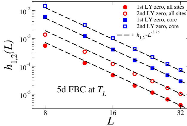
Figure 6. (Color online) The first two Lee-Yang zeros for Ising systems with FBC's at pseudocriticality obey Q-FSS whether the full lattice or only the core sites are used in their determination (see also figure 8 (c) of reference [4]).
