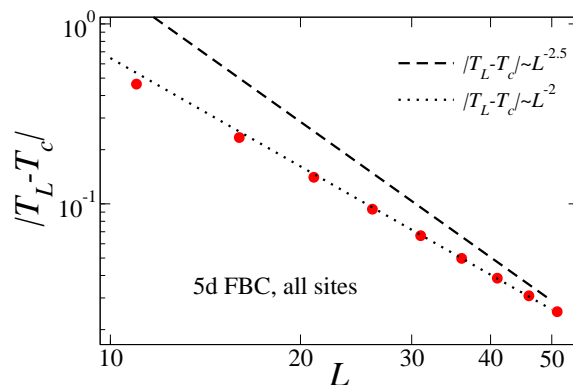
Figure 5. (Color online) The high-dimensional Ising shift exponent \lambda for FBC’s comes from the Gaussian formula \lambda = 1/\nu = 2 . This means that the shifting is bigger than the rounding in the FBC case, and the critical point T_c is too far from the pseudocritical point T_L to come under its scaling effect (see also figure 6 (b) of reference [4]).
