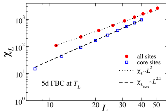
Figure 1. (Color online) FSS for the pseudocritical Ising susceptibility calculated on 5D lattices using all sites (upper data set, in red) and using only core sites (lower data, in blue). The upper data set appears to scale as \chi_L \sim L^2 , indicative of Gaussian FSS, but this is spurious and due to the preponderance of surface sites. The lower data, which are genuinely five-dimensional, scale according to the Q-FSS form \chi_L \sim L^{5/2} , supporting the universality of \varphi (see also figure 4 (a) of reference [4]).
