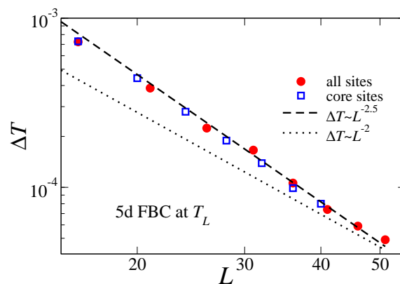
Figure 3. (Color online) FSS of the susceptibility rounding is compatible with the Q -FSS \theta = \vartheta/\nu = 5/2 rather than with the Gaussian FSS \theta = 1/\nu = 2 .
