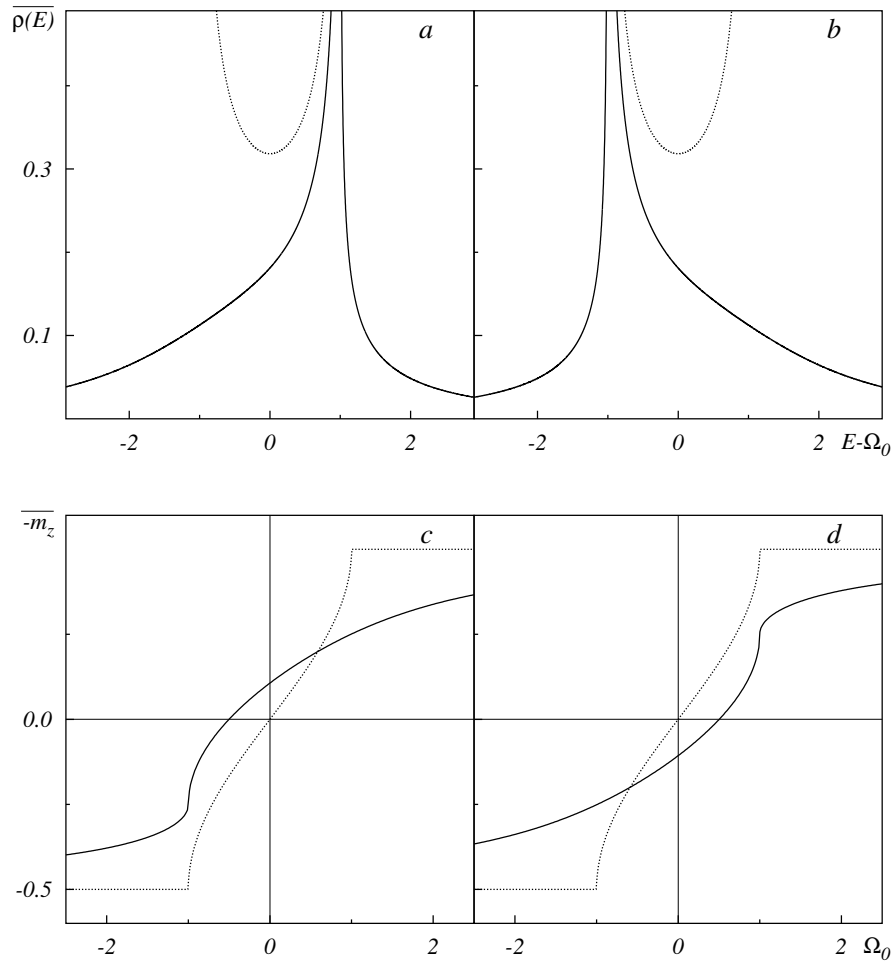
Figure 2. The density of states (a, b) and the transverse magnetization (c, d) of the isotropic XY chain with correlated Lorentzian disorder ( J_0 = 1 , \Gamma = 1 , a = -1 (a, c), a = 1 (b, d)). The dotted curves correspond to the nonrandom case ( \Gamma = 0 ).
