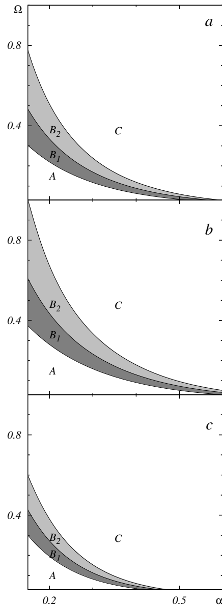
Figure 4. The phase diagram of the isotropic XY chain ( J = 1 ) in the plane lattice stiffness \alpha – transverse field \Omega which indicates the regions of stability/metastability of the dimerized and uniform phases at zero temperature. A (C) – only dimerized (uniform) phase occurs; B_1 ( B_2 ) both phases are possible but the dimerized (uniform) is the favourable one. The phase diagram also illustrates the possible effects of the Dzyaloshinskii-Moriya interaction (a: D = 0 , b: D = 0.5 , k = 1 , c: D = 0.5 , k = 0 ).
