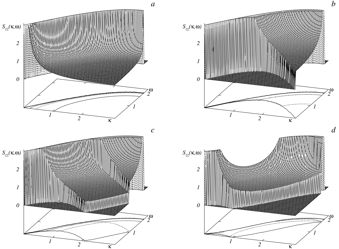
Figure 1. S_{zz}(\kappa, \omega) for the isotropic XY chain in a transverse field ( J = 1 ) at infinite temperature \beta = 0 (a) and zero temperature \beta \rightarrow \infty (b: \Omega = 0 , c: \Omega = 0.5 , d: \Omega = 0.9 ).
