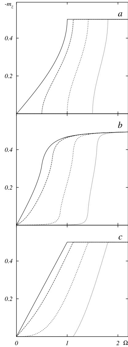
Figure 3. The zero-temperature magnetization curves for the isotropic XY (a), transverse Ising (b) and classical (c) chains of period 2 ( J_n = 1 , \Omega_{1,2} = \Omega \pm \Delta\Omega , \Delta\Omega = 0 (solid curves), \Delta\Omega = 0.5 (long-dashed curves), \Delta\Omega = 1 (short-dashed curves), \Delta\Omega = 1.5 (dotted curves)).
