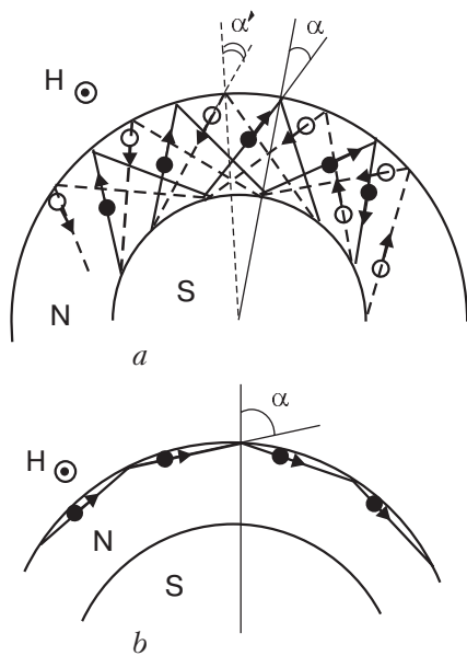
Fig. 1. Two classes of trajectories in the normal metal of NS structure in the magnetic field: trajectories forming the Andreev levels (a); trajectories colliding only with the dielectric boundary (b).
