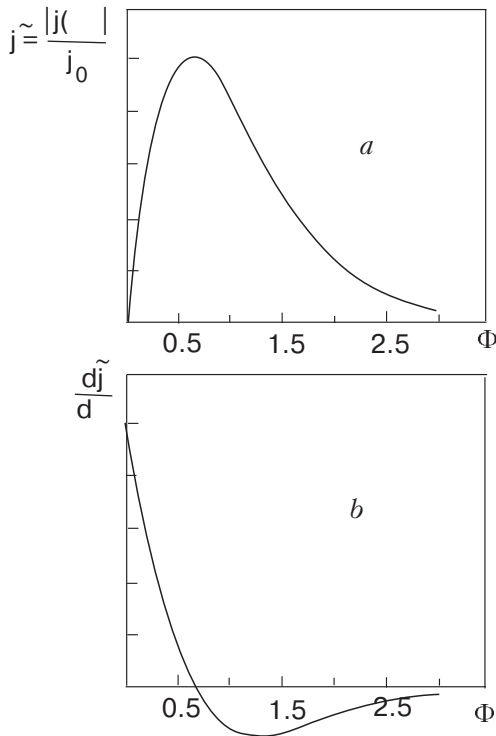
Fig. 2. Dependence of screening current Eq. (5) on «phase» \Phi at T = 0.092 K. Current is in arbitrary units (a). The derivative of current with respect to «phase» (magnetic field) changes its sign in the region of low \Phi -values (b). When the magnetic field tends to zero the full magnetic susceptibility of NS structure is positive for d = 3.3 \cdot 10^{-4} cm.
