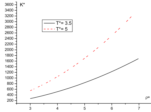
Figure 5. Density dependence of the elasticity constant.
