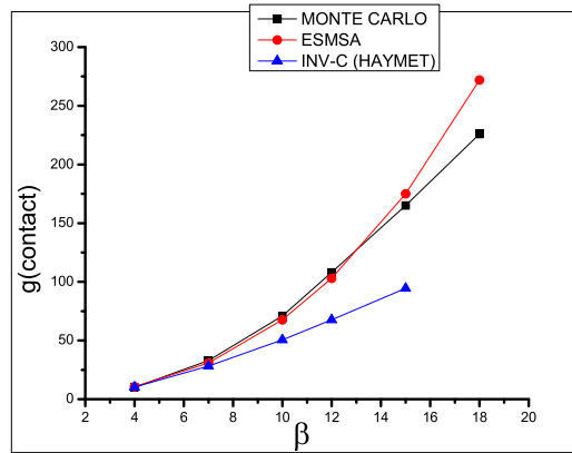
Figure 1. Comparison of the contact pair distribution function for g_{+-}^{\text{ESMSA-BIMSA}} . The squares are the Monte Carlo results by Bresme et al. [22]. The triangles are the INV-C theory of Haymet et al [25]. The circles are the ESMSA-BIMSA with \eta = 0 and an effective dielectric constant of \epsilon_0 = 1.17 (which also depends on the association constant \alpha ).
