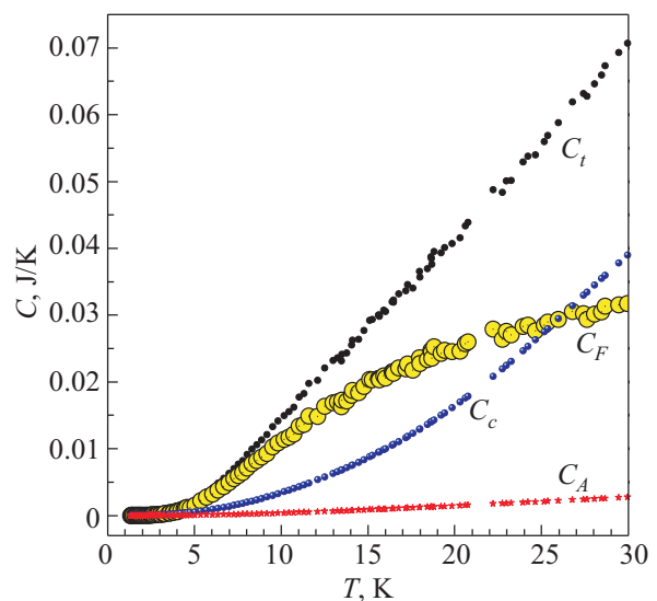
Fig. 4. The total heat capacity C_t of the calorimeter with the sample, the heat capacities of the empty calorimeter C_c , the sample C_F and grease Apiezon C_A .
