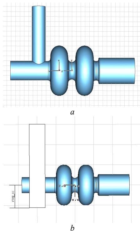
Fig.1. Coaxial and waveguide input couplers
