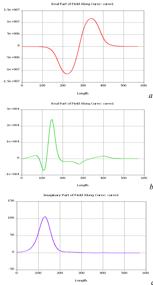
Fig.2. Longitudinal (a), transverse (b) components of electric field and transverse component of magnetic field (c) on structure axis with electric wall boundary condition usage
