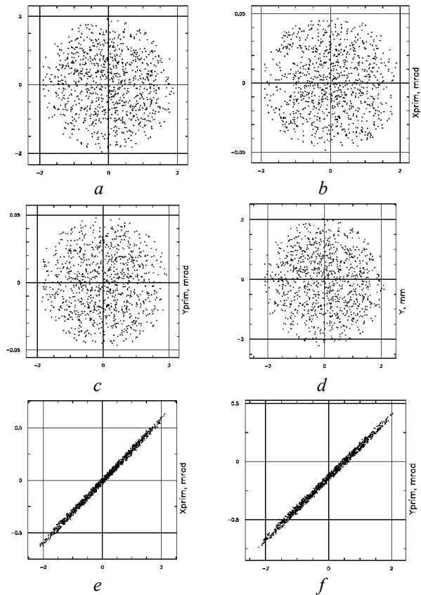
Fig.3. Beam parameters before (a – cross-section, b – phase plane x-xp, c – phase plane y-yp) and after passing the accelerator (d – cross-section, e – phase plane x-xp, f – phase plane y-yp)
