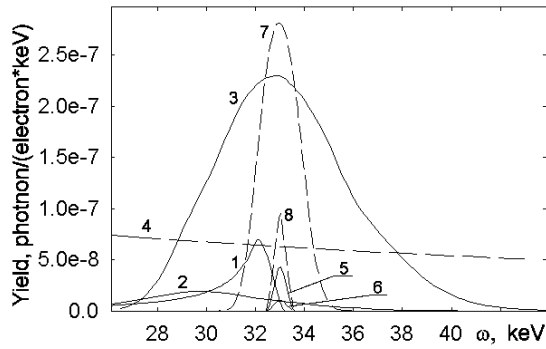
Fig.3. Radiation spectra for the pyrolytic graphite crystals. E_e=45 MeV, \vartheta_c=1 mrad. Curves: 1-PXR spectrum in the perfect crystal; 2-PXR spectrum in the mosaic crystal; 3-DB spectrum in the mosaic crystal; 4-BS spectrum on the flying into the second crystal; 5-the spectrum of double diffracted radiation; 6-the spectrum of the diffracted BS. 7-DB spectrum in the crystal with \sigma_m=1 mrad and T_1=5 mm; 8-The spectrum after the second crystal with \sigma_m=1 mrad and T_2=4 mm
