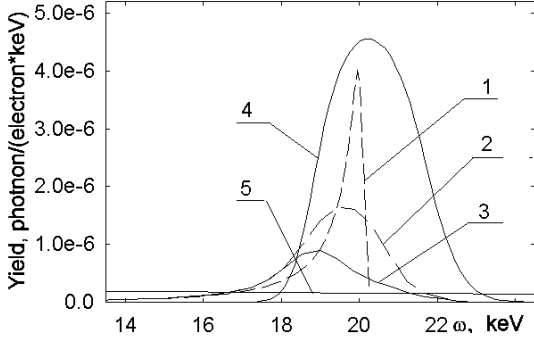
Fig.2. Radiation spectra in the mosaic crystal of pyrolytic graphite for the conditions of the work [6]
